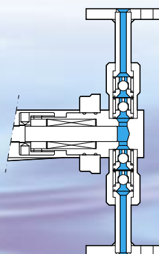
Plunger
