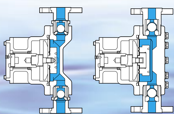
Mechanically-driven diaphragm
